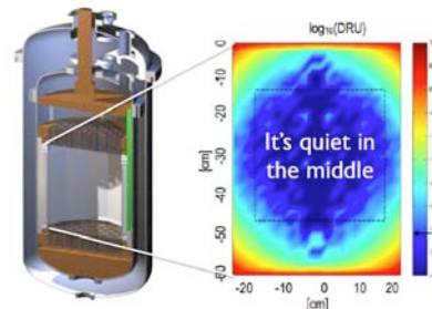
Figure 2: Left: Cross-section of the LUX detector. 350 kg liquid xenon volume delimited at top and bottom by two arrays of photo detectors (dark grey). The detector is composed of two concentric Titanium shells, the inner one at liquid xenon temperature (165 K or -162 F), and the outer one providing vacuum thermal insulation. Right: Results of background simulation showing the center of the detector at four orders of magnitude quieter than its edges. By identifying and selecting only events occurring in the center of the detector, LUX gets rid of much background and increases chances of observing rare dark matter interactions.
